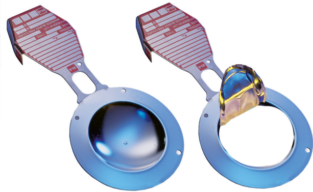
The Fail-safe CSI™ Reverse Buckling Disk
