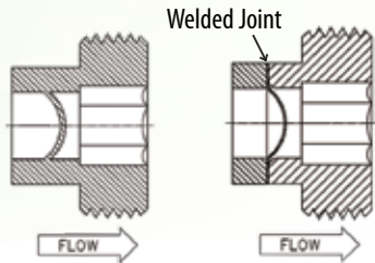
Left: XTI Integral Assembly
